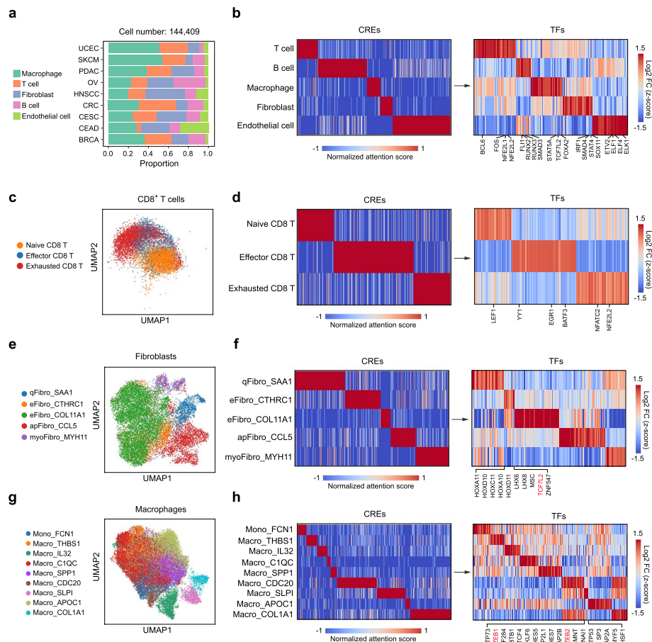
Fig. 4 Cisformer uncovers cell-type-specific regulatory programs in the tumor microenvironment. a Barplots showing the relative cell proportion in nine different cancer types. Total cell number is listed at the top. UCEC, uterine corpus endometrial carcinoma; SKCM, skin cutaneous melanoma; PDAC, pancreatic ductal adenocarcinoma; OV, ovarian cancer; HNSCC, head and neck squamous cell carcinoma; CRC, colorectal cancer; CESC, cervical squamous cell carcinoma; CEAD, cervical adenocarcinoma; BRCA, breast cancer. b Heatmaps illustrating the normalized attention score of CREs (left) and motif enrichment of TFs (right) in five major cell types (T cells, B cells, macrophages, fibroblasts, and endothelial cells). TFs associated with the regulation of respective cell functions are marked below the heatmap. c UMAP visualization of CD8 + T cell subtypes (CD8 + naïve T cell, CD8 + effector T cell, and CD8 + exhausted T cell). d Heatmaps showing the CRE normalized attention score (left) and TF motif enrichment (right) in CD8 + T cell subtypes. TFs regulating each cell subtype's function are labeled below the heatmap. e UMAP visualization of five fibroblast subtypes. f Heatmaps displaying cell-type-specific CREs (left) and TFs (right) in fibroblast subtypes. Inferred TFs that regulate cellular function of CTHRC1 + ECM-remodeling fibroblasts (eFibro_CTHRC1) are listed below the heatmap. g UMAP visualization of nine macrophage subtypes. h Heatmaps showing cell-type-specific CREs (left) and TFs (right) in macrophage subtypes. Predicted TFs involved in the regulation of SLPI + macrophage (Macro_SLPI) are listed below the heatmap
