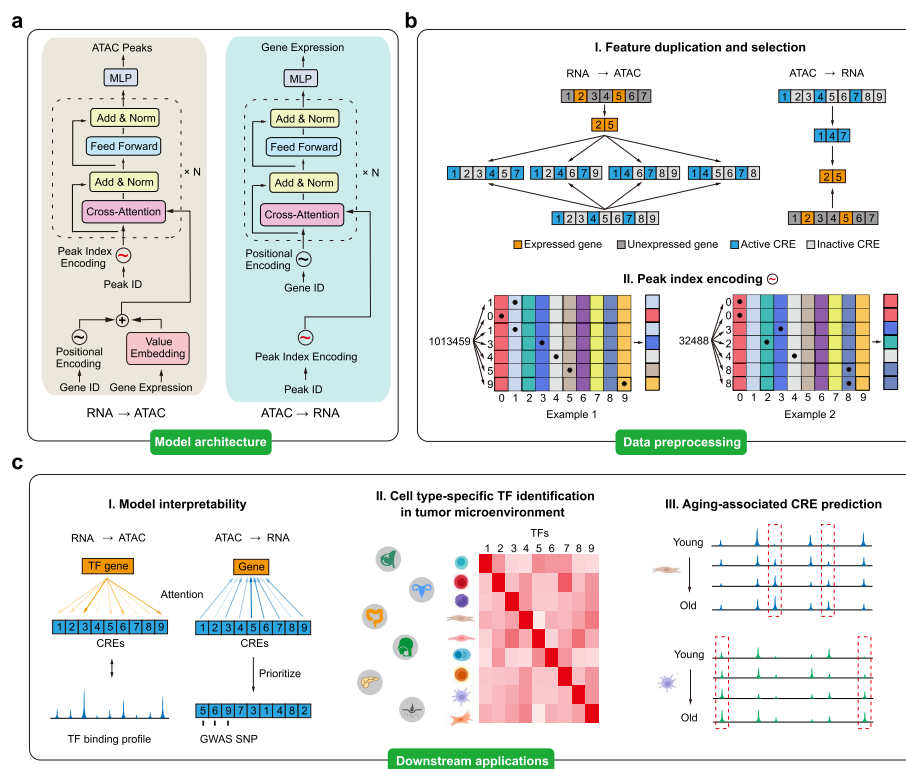
Fig. 1 Overview of the Cisformer model. a The model architecture of Cisformer for single-cell RNA-to-ATAC (left) and ATAC-to-RNA (right) generation. Gene and peak features are encoded respectively, integrated through Transformer blocks with cross-attention mechanisms, and subsequently transformed into final outputs by an MLP. b The genes and chromatin peaks are selected or duplicated to generate gene-peak pairs as model input (top). Chromatin peak indices are encoded through a digit decomposition strategy, with 1,013,459 and 32,488 as representative examples (bottom). c The downstream applications of Cisformer, including validating biological interpretability (left), identifying cell-type-specific TFs in pan-cancer datasets (middle), and predicting aging-related CREs (right)
